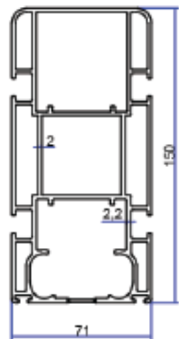
PROFILE NO 6413 WEIGHT 4.655 KG/M
