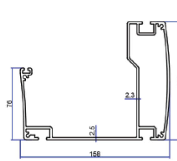
PROFILE NO 5935 WEIGHT 3.918 KG/M
