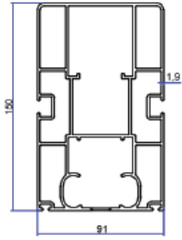
PROFILE NO 2052 WEIGHT 5.217 KG/M
