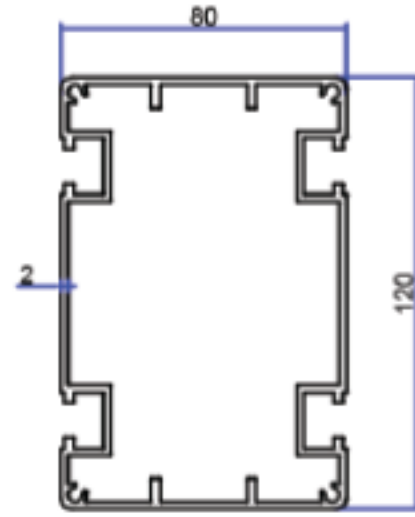
PROFILE NO 5936 WEIGHT 3.032 KG/M
