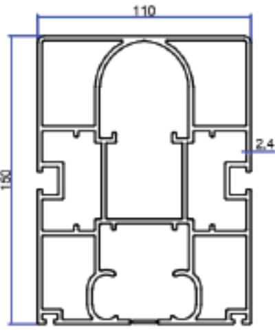
PROFILE NO 2001 WEIGHT 7.168 KG/M
