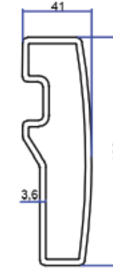
PROFILE NO 2281 WEIGHT 3.246 KG/M
