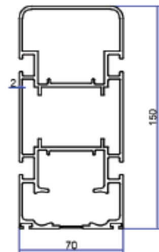
PROFILE NO 5922 WEIGHT 4.212 KG/M
