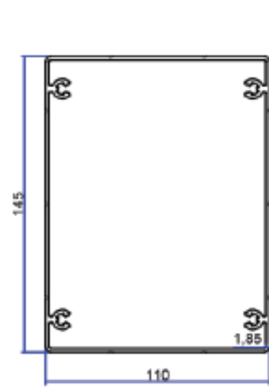
PROFILE NO 2111 WEIGHT 3.044 KG/M
