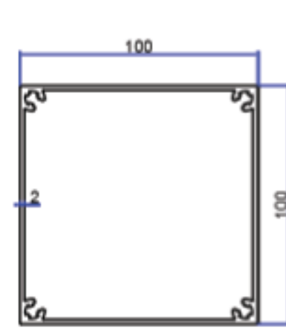
PROFILE NO 2111 WEIGHT 3.044 KG/M
