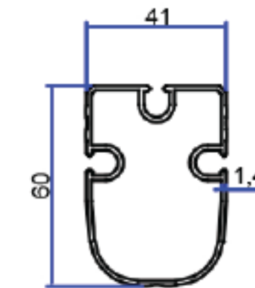
PROFILE NO 37153 WEIGHT 0.937 KG/M
